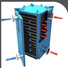
Cubic WPHE - corruguated / free gap
