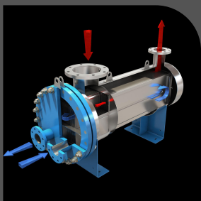
Cylindrical WPHE - free gap
