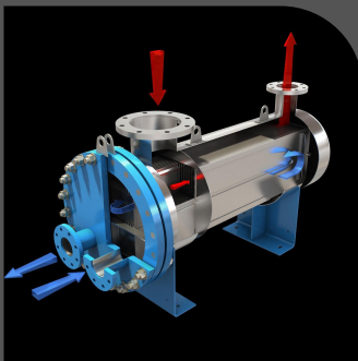
Cylindrical WPHE - free gap
