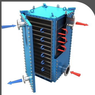
Cubic WPHE - corrugated / free gap
